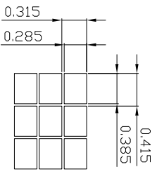
DETAIL "A" (S=10:1)
